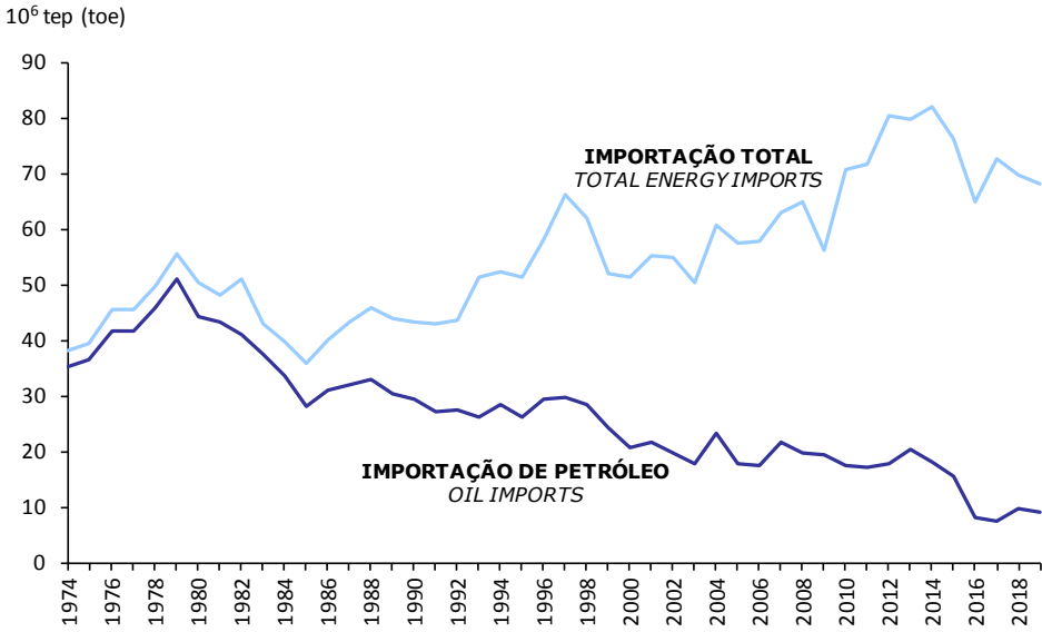
Chart 4.3 – Energy Imports
