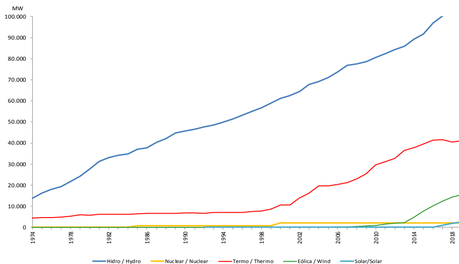
Chart I.1 – Installed Capacity Of Electric Energy Generation
