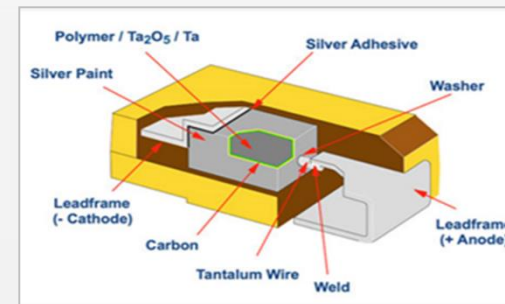
Tantalum Capacitor
