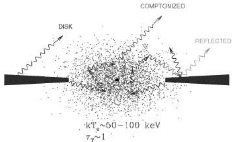
Fig. 2.2 The three main components of the X-ray emission from an accreting black hole ( top ) and a plausible geometry of the accretion flow in the hard spectral state ( bottom )
