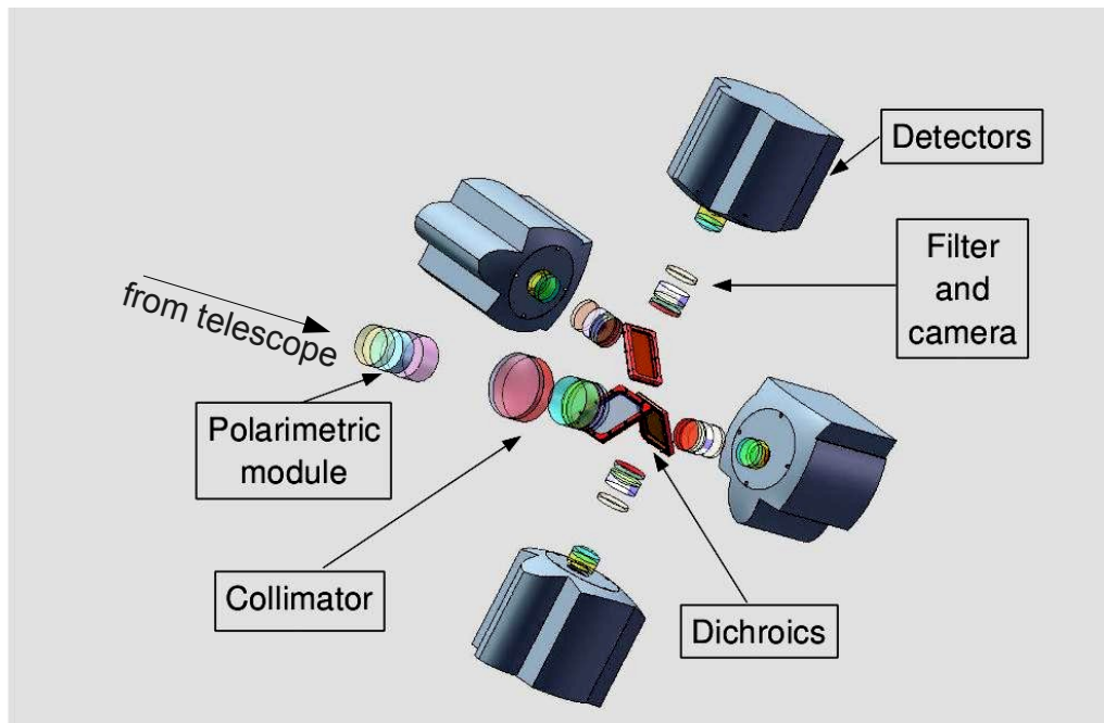
FIGURE 1. SPARC4 layout.
