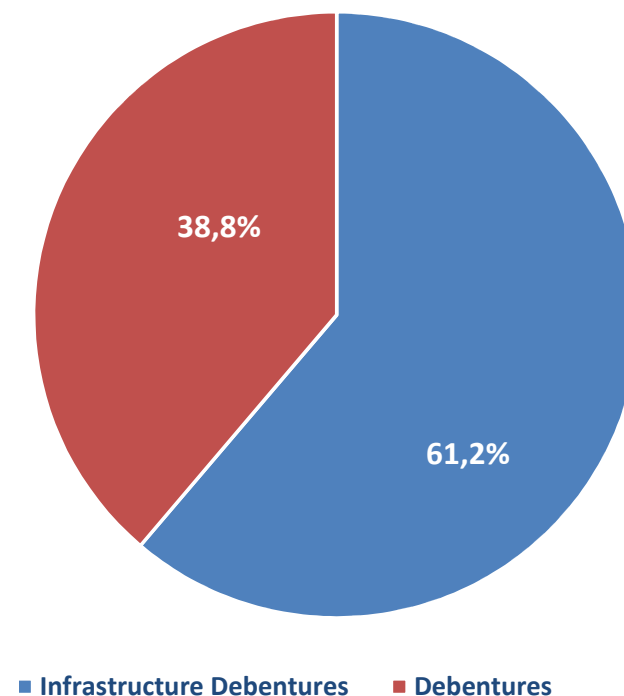
Share of Trades May/2016 to May/2018
