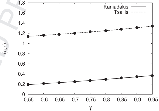
Fig. 6. Expressions \kappa = \kappa(\gamma) and q = q(\gamma) were obtained in the best fit calculated in Fig. 5. We can see an exponential behavior increasing smoothly unlike that one shown in Fig. 5. The exponential behavior is given by the best fits expressed by solid curve \kappa = -0.179 + 0.216e^{0.983\gamma} and the dashed curve q = 0.868 + 0.127e^{1.382\gamma} .
