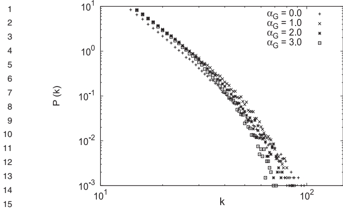
Fig. 1. This panel shows numerical curves for degree distribution for \alpha_A = 2 and typical values of \alpha_G for networks of size N = 10^4 sites. This parameter has influence in the growth of network.
