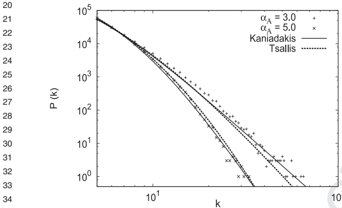
Fig. 2. Curves for degree distribution for typical values of \alpha_A for networks of size 2 \times 10^6 . Points are our computer simulation results, solid lines are the best fit given by P(k) = P_0 \exp_{\kappa}(-k/\eta_{\kappa}) and dashed lines are the best fit given by P(k) = P_0 \exp_q(-k/\eta_q) . This panel shows the log-log representation.
