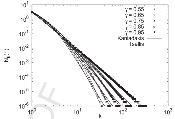
67 68 69 70 71 72 73 74 75 76 77 78 79 80 81 82 83 84 85 86 87 88 89 90 91 92 93 94 95 96 97 98 99 100 101 102 103 104 105 106 107 108 109 110 111 112 113 114 115 116 117 118 119 120 121 122 123 124 125 126 127 128 129 130 131 132 Fig. 5. Analytical curves for the degree distribution in the interval 1/2 < \gamma < 1 . Points are obtained of the analytical expression N_k(t = 1) vs k . The solid lines are the best fit given by N_k(1) = N_0 \exp_\kappa(-k/\eta_\kappa) and dashed lines are the best fit given by N_k(1) = N_0 \exp_q(-k/\eta_q) . This panel shows the log–log representation.
