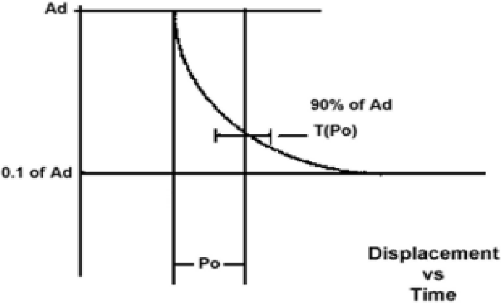
Attachment 2 to Appendix D to Part 60— Figure D2B. Critically-Damped Step Response
