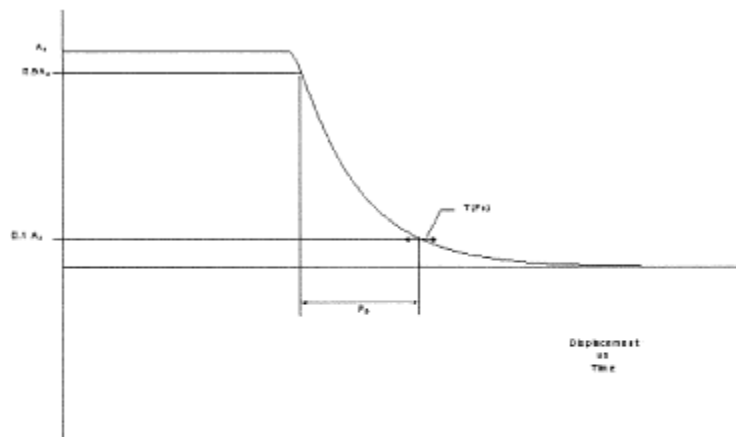
Figure A2A Underdamped Step Response
