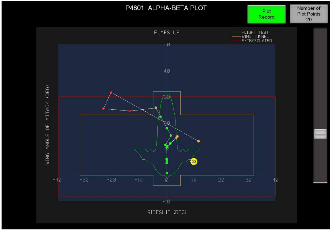
Figure 1 – Example FSTD Alpha/Beta Envelope Plot
