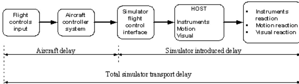
Figure C2F Transport Delay for simulation of Computer Controlled Aircraft using real helicopter black boxes
