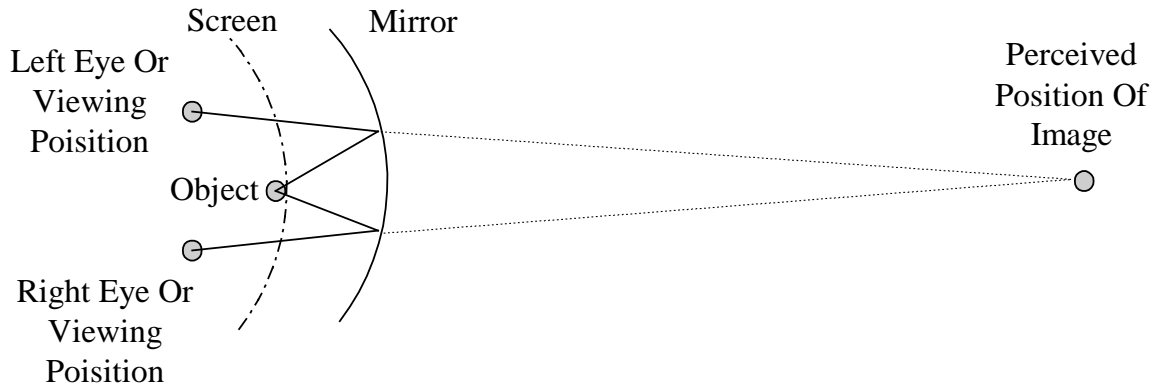
Figure C2I - Collimated display
