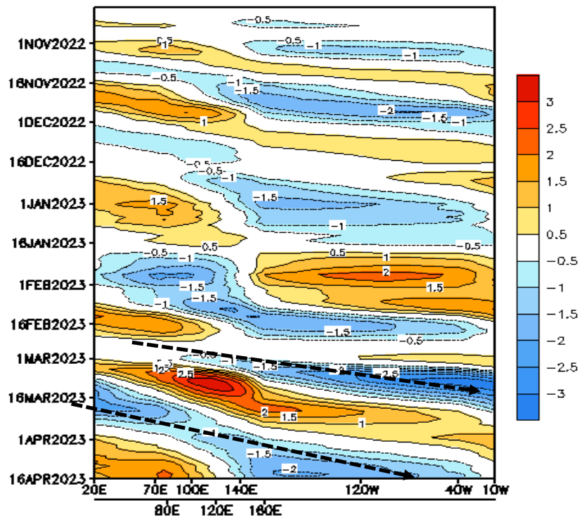
5 -day Running Mean
