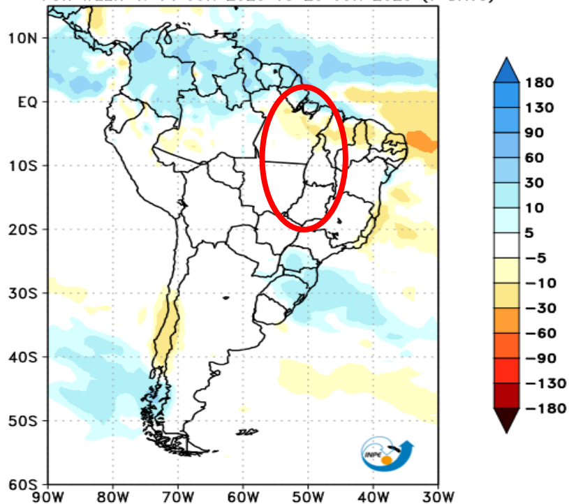
CPTEC/INPE (BAM1.2) PRECIPITATION ANOMALY (mm) FORECAST ISSUED: 24 MAY 2023 FOR WEEK 4: 14 JUN 2023 TO 20 JUN 2023 (7 DAYS)
