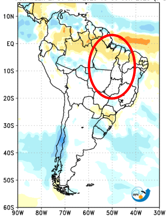
CPTEC/INPE (BAM1.2) PRECIPITATION ANOMALY (mm) FORECAST ISSUED: 24 MAY 2023 FOR WEEK 2: 31 MAY 2023 TO 06 JUN 2023 (7 DAYS)
