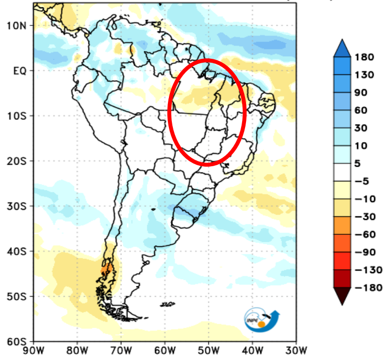
CPTEC/INPE (BAM1.2) PRECIPITATION ANOMALY (mm) FORECAST ISSUED: 24 MAY 2023 FOR WEEK 3: 07 JUN 2023 TO 13 JUN 2023 (7 DAYS)
