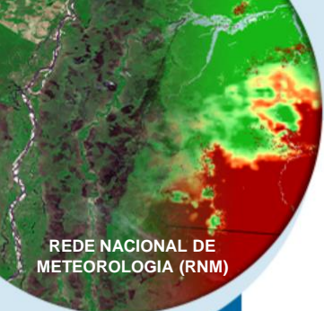
CPTEC/INPE (BAM1.2) PRECIPITATION ANOMALY (mm) FORECAST ISSUED: 24 MAY 2023 FOR WEEK 2: 31 MAY 2023 TO 06 JUN 2023 (7 DAYS)
