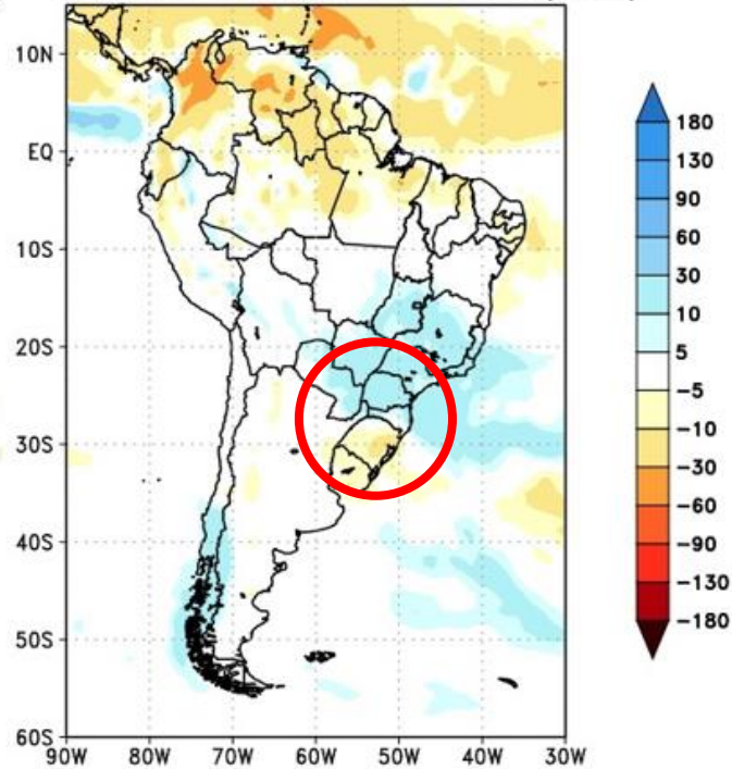
CPTEC/INPE (BAM1.2) PRECIPITATION ANOMALY (mm) FORECAST ISSUED: 16 AUG 2023 FOR WEEK 3: 30 AUG 2023 TO 05 SEP 2023 (7 DAYS)
