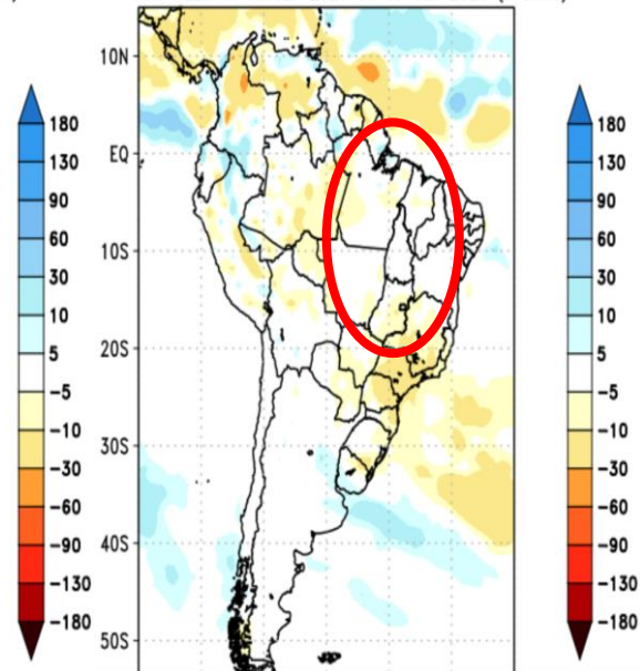
CPTEC/INPE (BAM1.2) PRECIPITATION ANOMALY (mm) FORECAST ISSUED: 23 AUG 2023 FOR WEEK 4: 13 SEP 2023 TO 19 SEP 2023 (7 DAYS)
