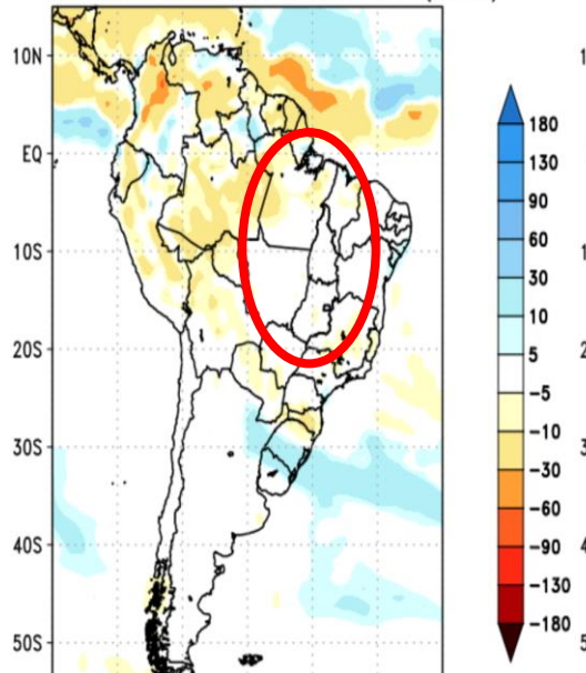
CPTEC/INPE (BAM1.2) PRECIPITATION ANOMALY (mm) FORECAST ISSUED: 23 AUG 2023 FOR WEEK 3: 06 SEP 2023 TO 12 SEP 2023 (7 DAYS)
