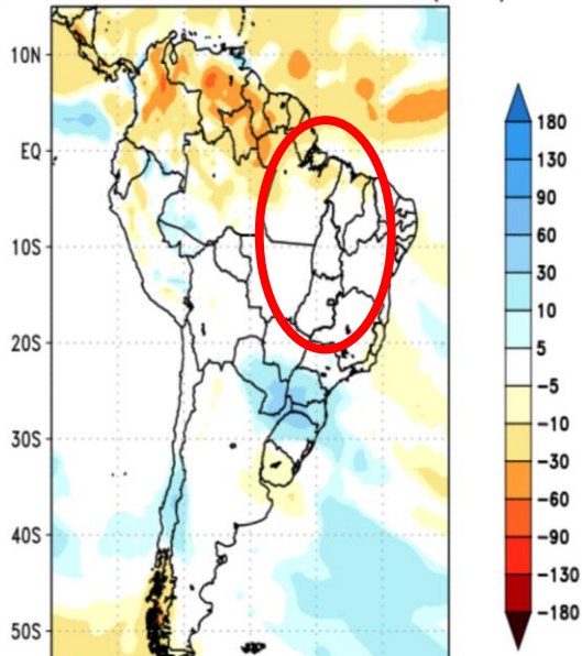
CPTEC/INPE (BAM1.2) PRECIPITATION ANOMALY (mm) FORECAST ISSUED: 23 AUG 2023 FOR WEEK 2: 30 AUG 2023 TO 05 SEP 2023 (7 DAYS)
