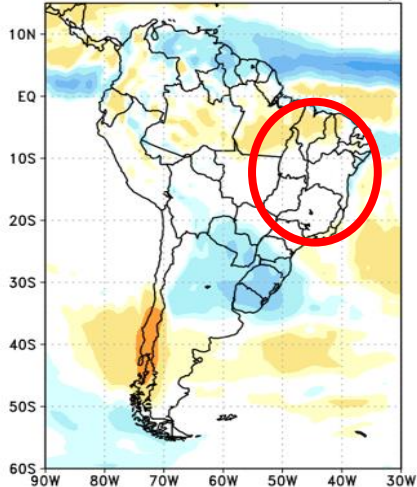
CPTEC/INPE (BAM1.2) PRECIPITATION ANOMALY (mm) FORECAST ISSUED: 31 MAY 2023 FOR WEEK 2: 07 JUN 2023 TO 13 JUN 2023 (7 DAYS)
